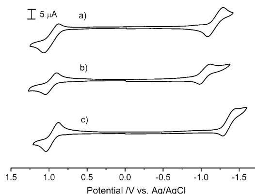
Figure 2. Cyclic voltammograms of a) 1 , b) 4 , and c) 6 in THF containing 0.1 M TBAPF 6 .
